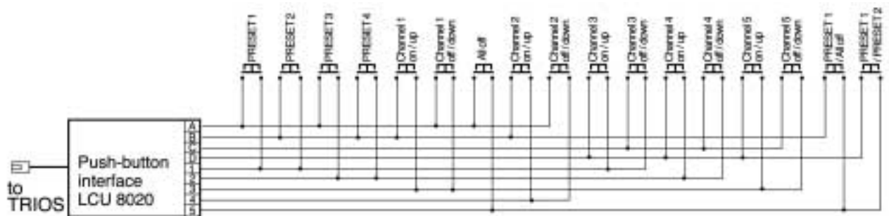
Figure 19: Switch combinations
