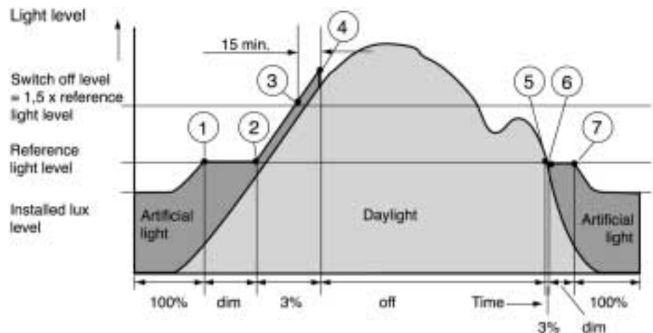
Figure 29: Regulation cycle for dimmable luminaires
