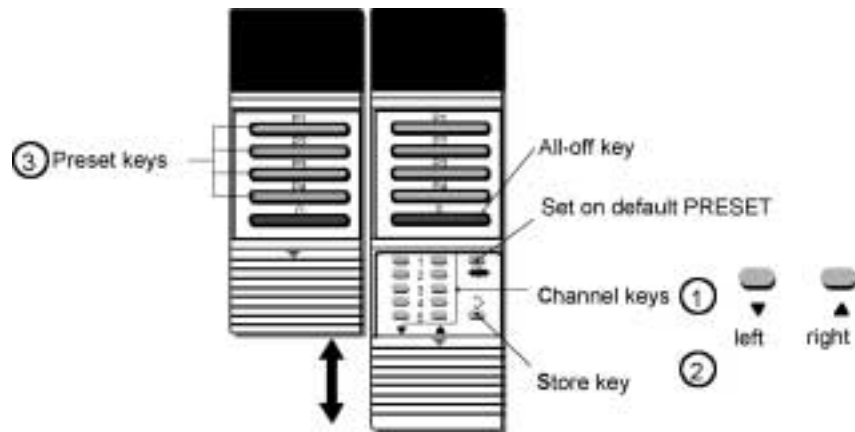
Figure 15: Function keys of the IR remote control IRC 2130
